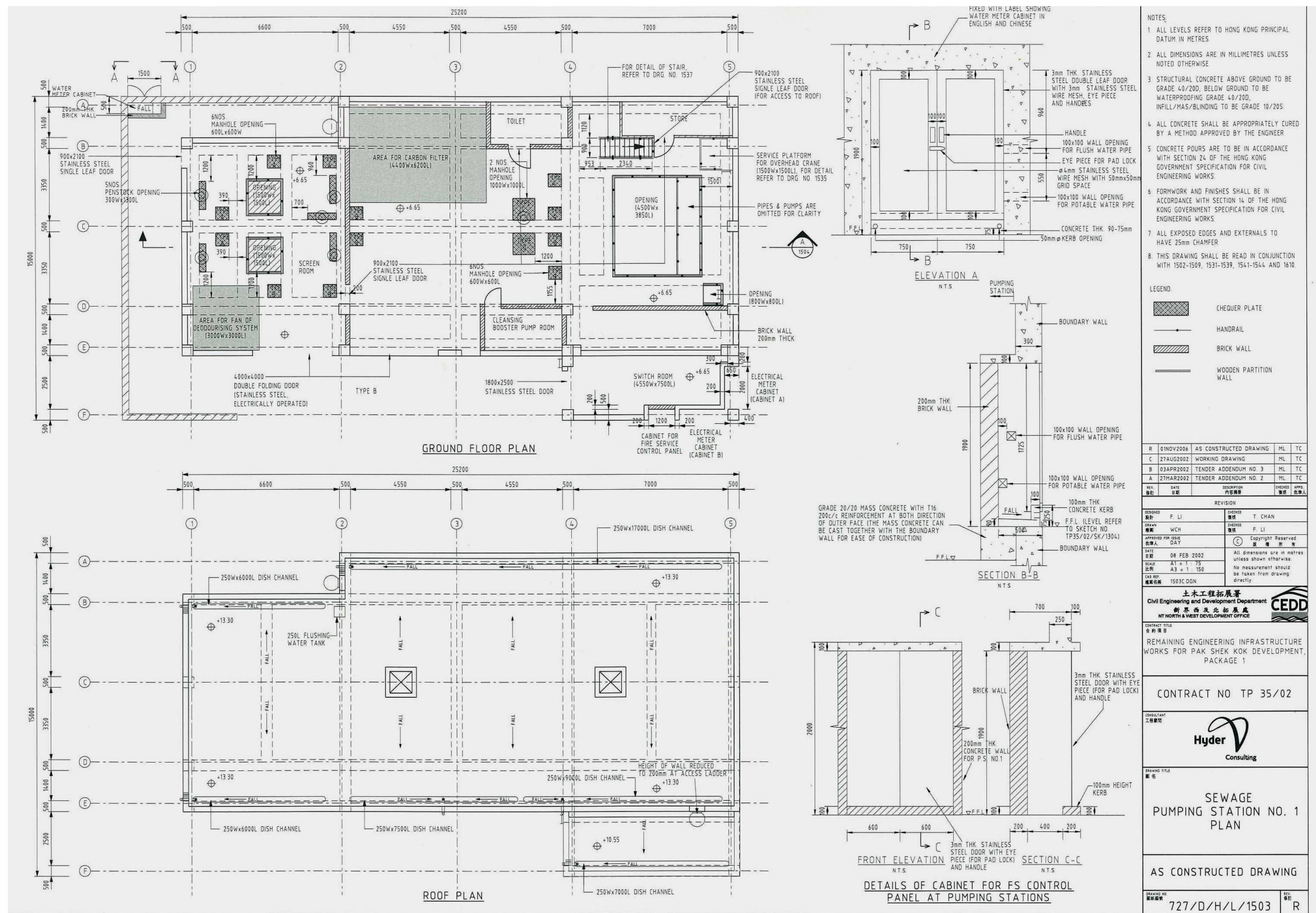
Figure 3: Sewage Pumping Station No. 1 Plan
